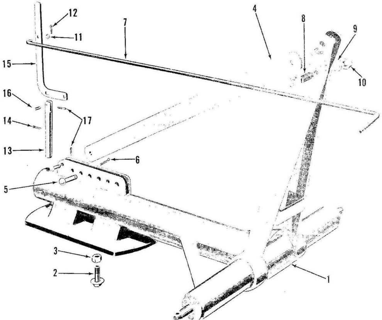
Fig. 11 - Frame Assembly 19-5
