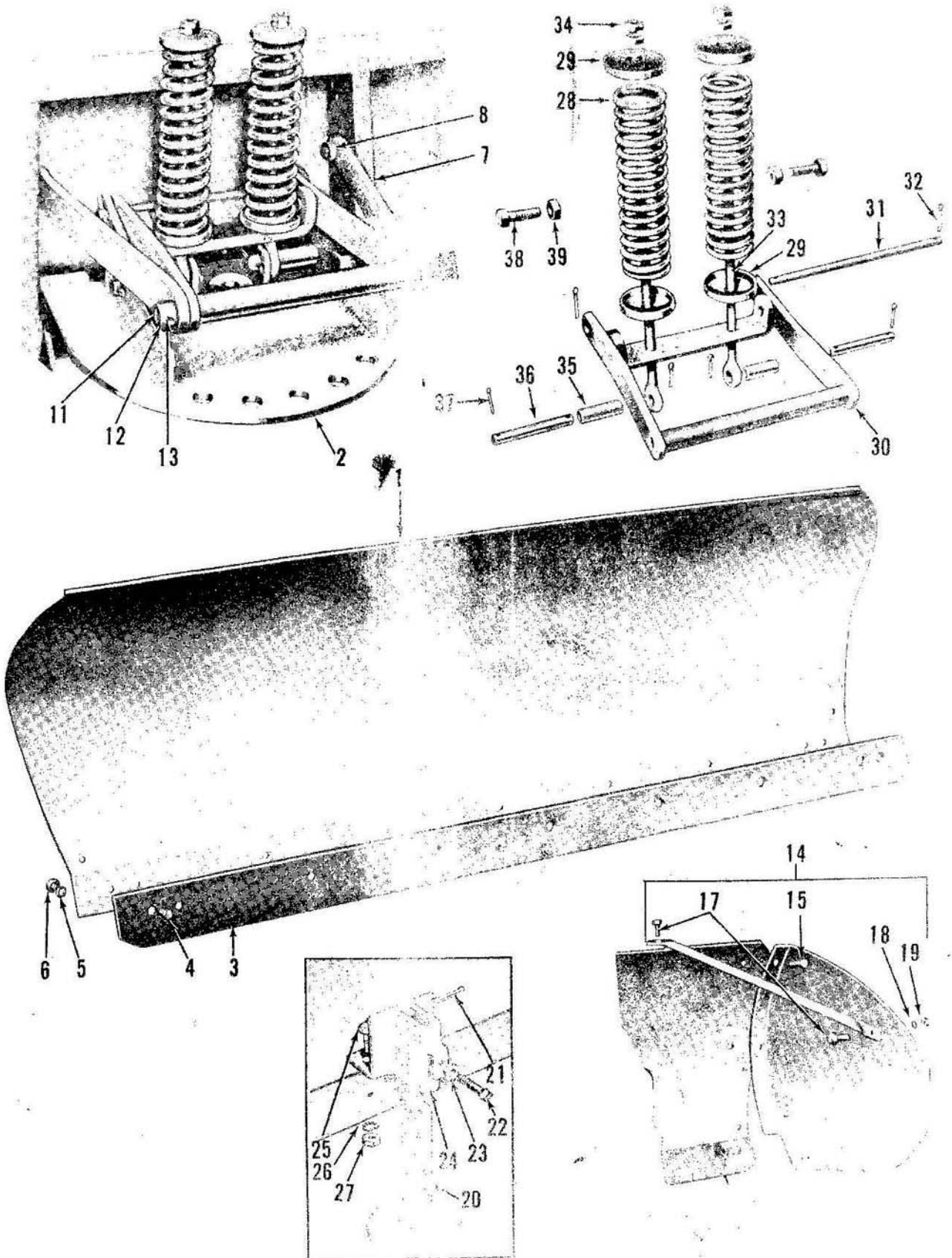
Fig. 9 - Blade, Release Spring, Plate
