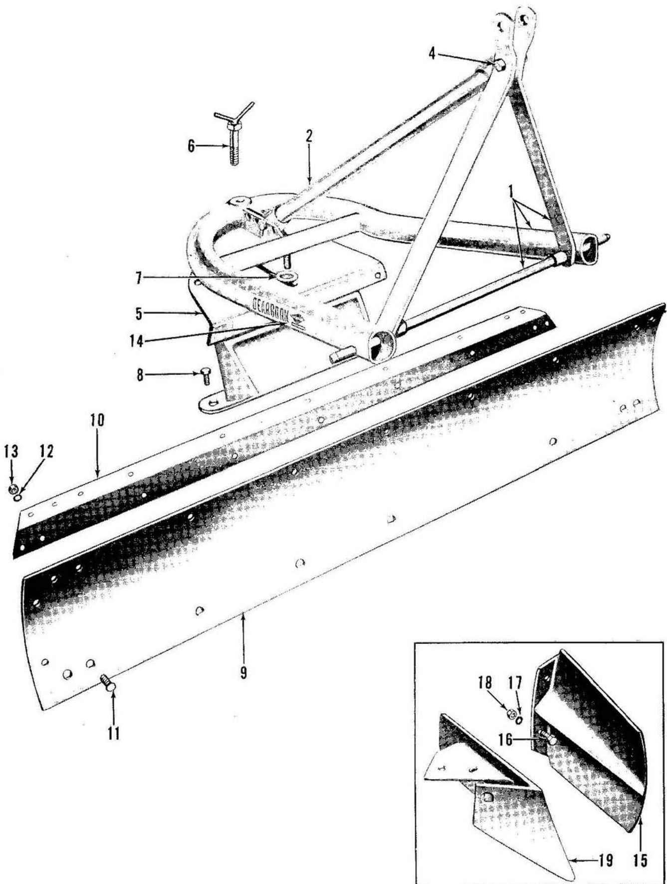
Fig. 14 - Frame, Blade & Attachments 19-72
