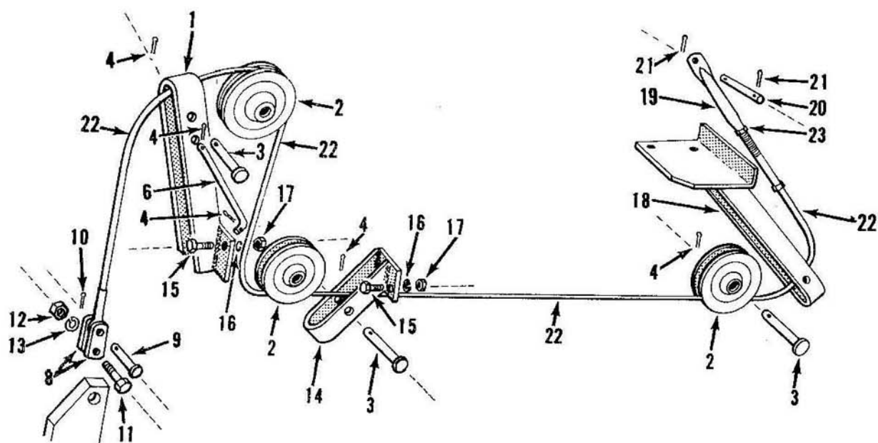
Fig. 7 - Hyd. Cable Control Attachment 19-441
