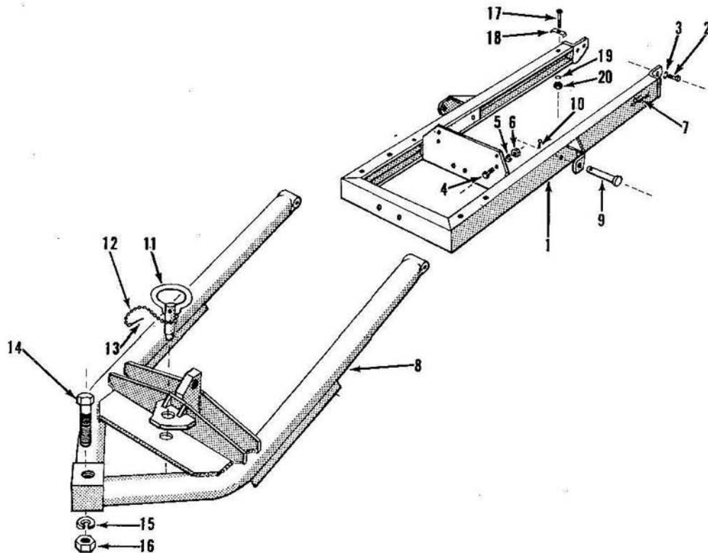
Fig. 3 - Dozer Frame - 19-439
