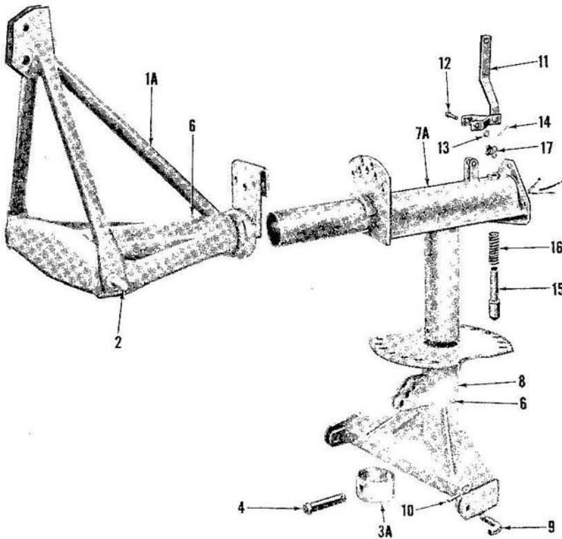
Fig. 15 - Frame & Turntable Parts 19-85,205
