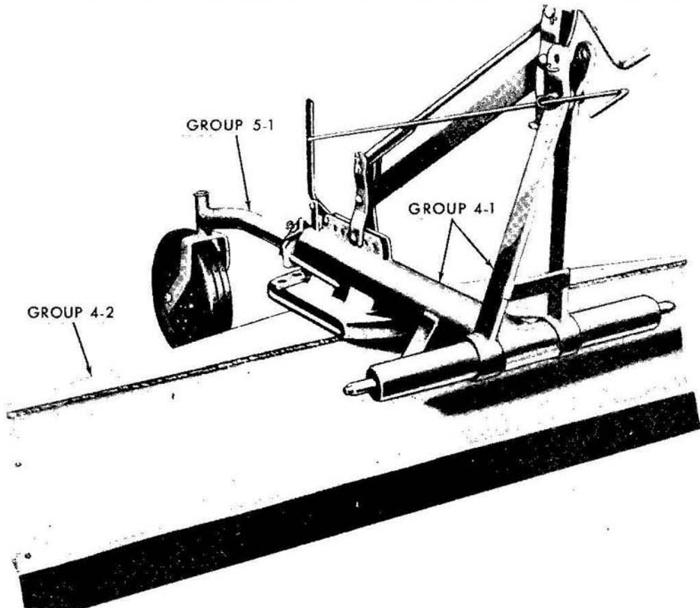
Fig. F - Dearborn Utility Blade 19-5 W/Gauge Wheel Attachment 19-19
