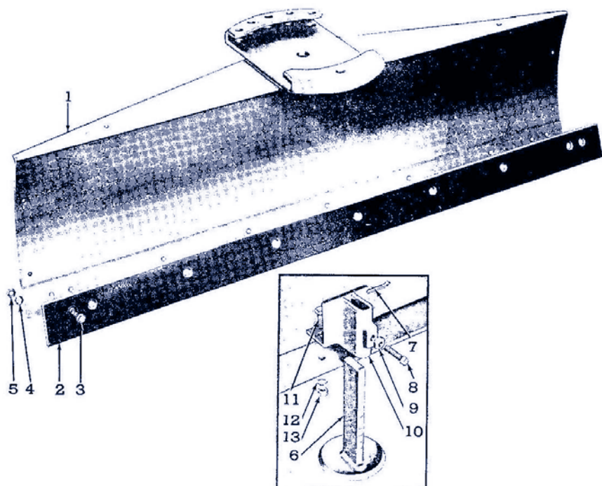
Fig. 12 - Blade Assembly With Skid Shoes 19-5
