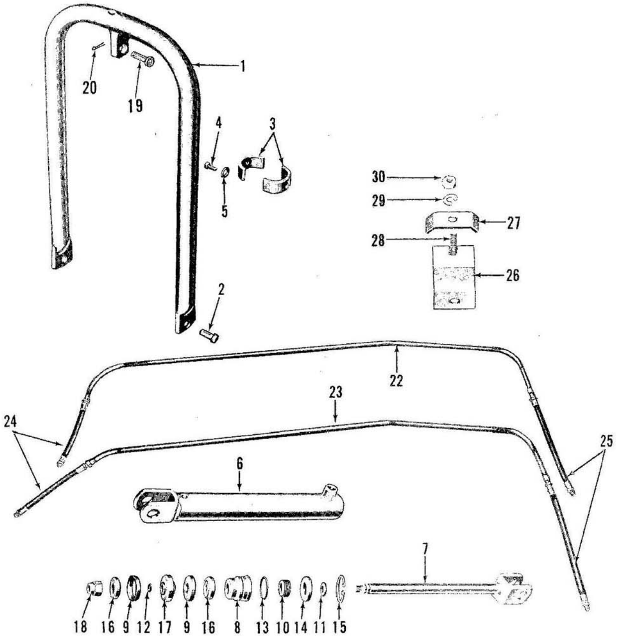
Fig. 4 - Hyd. Cylinder Control 19-91
