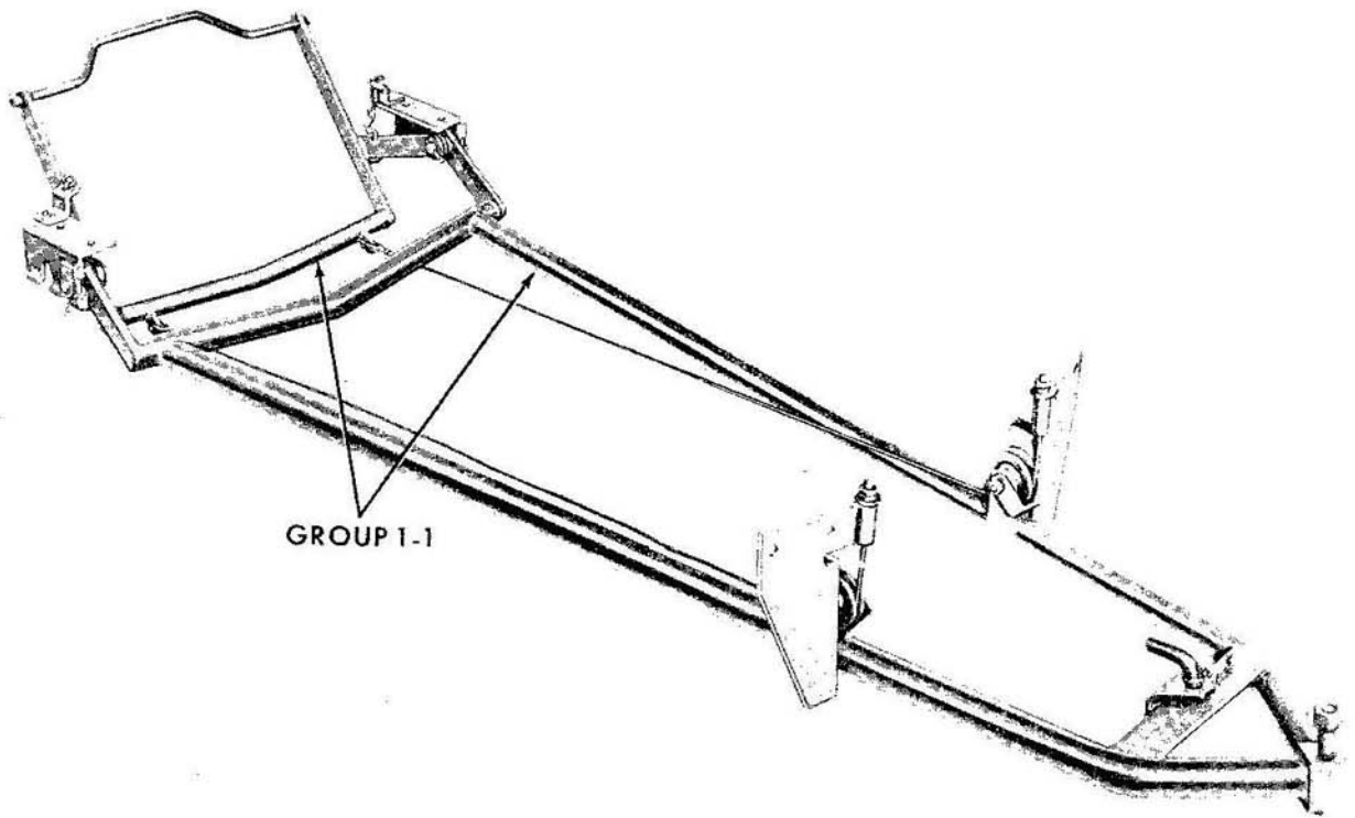
Fig. A - Dearborn Universal Frame 19-55,19-1
