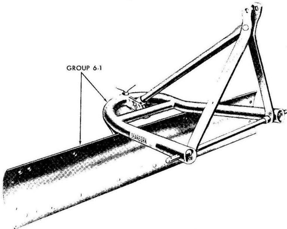
Fig. F - Dearborn Utility Blade 19-5 W/Gauge Wheel Attachment 19-19
