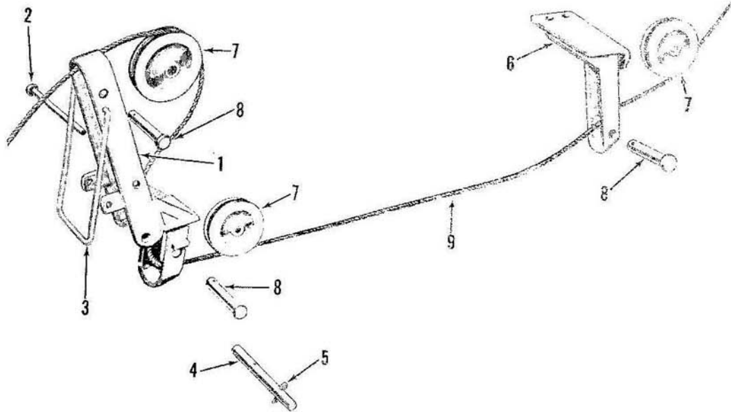
Fig. 6 - Hydraulic Cable Control Attachment 19-92
