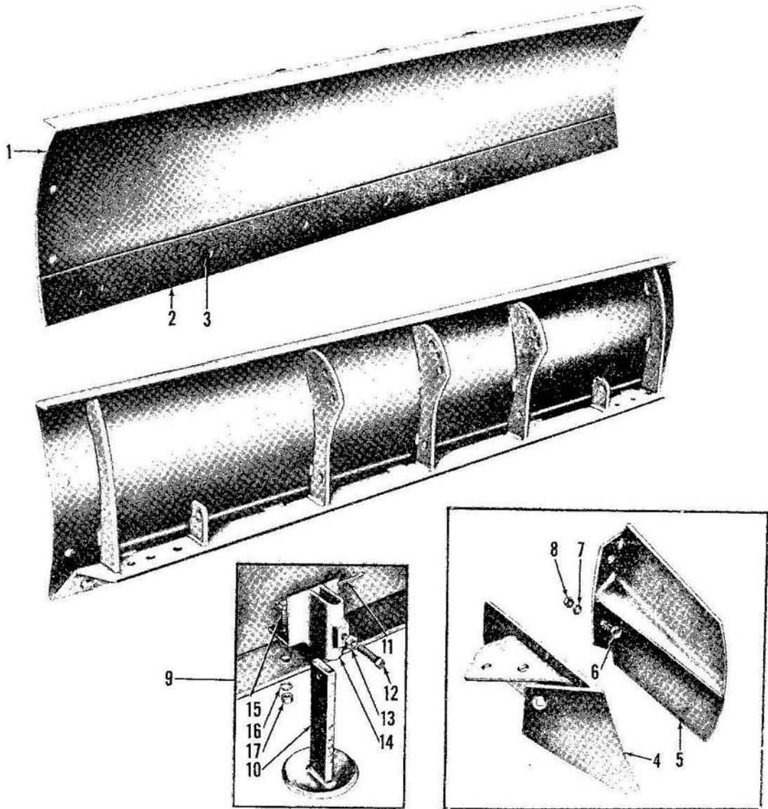
Fig. 16 - Blade Assembly
